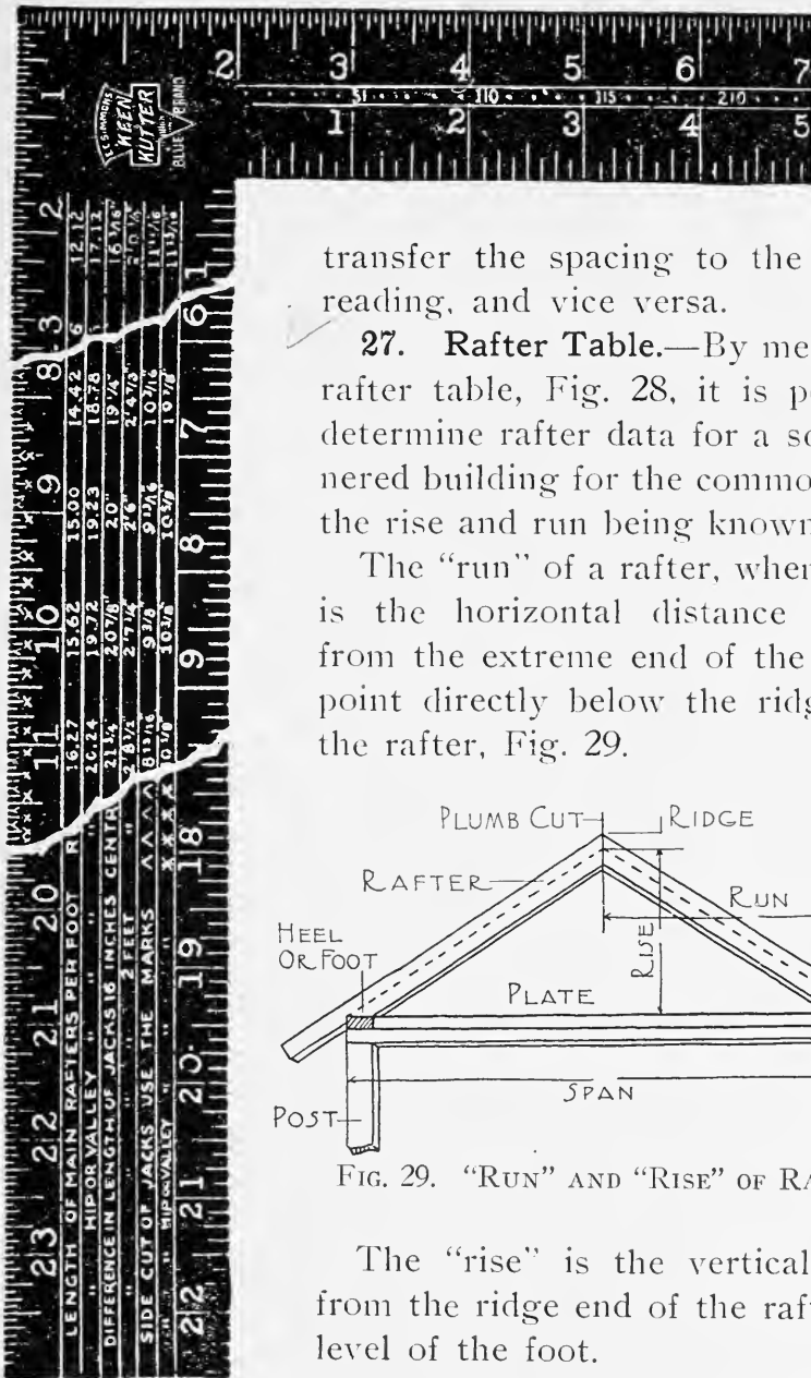
FIG. 28. NICHOLS' RAFTER TABLE.
